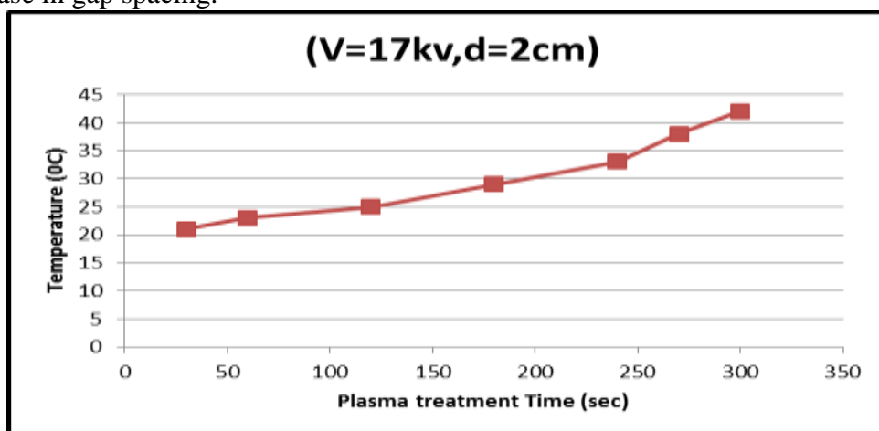
Figure (3): The temperature during the plasma treatment (under the operating conditions of a 17 kV applied voltage ,distance 2cm)
