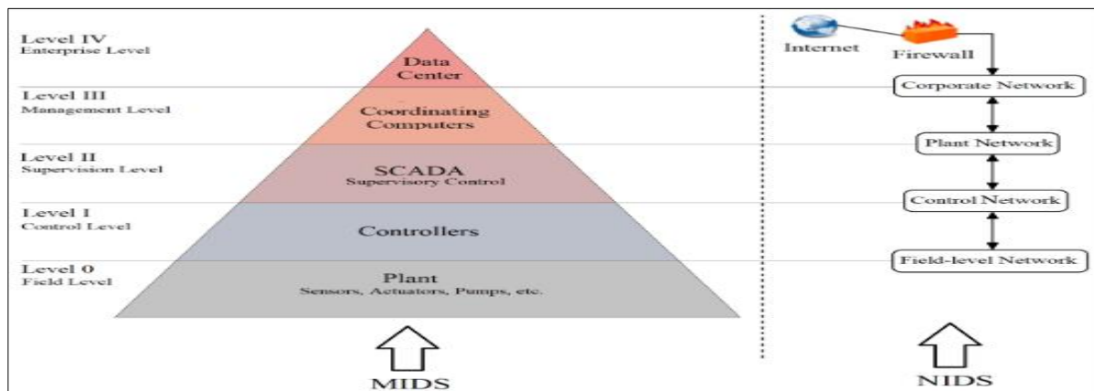
Figure 2: Anomaly detection architecture [8]
