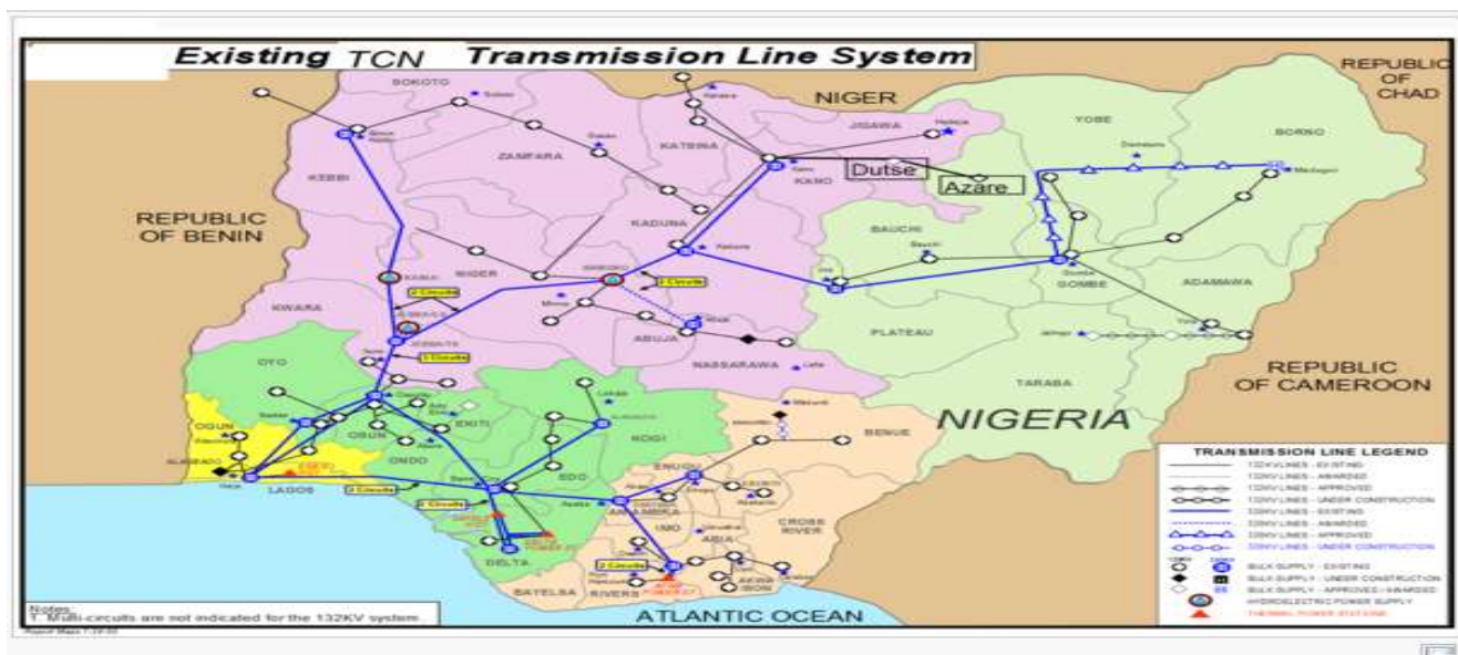
Fig 8: Transmission and Distribution Network in Nigeria.
