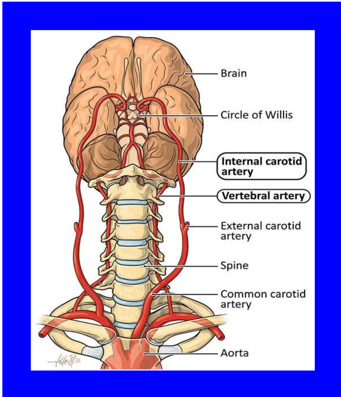
Figure 10: Two pairs of arteries named vertebral & carotid arteries that supply blood to brain (anterior or ventral view) [20].
